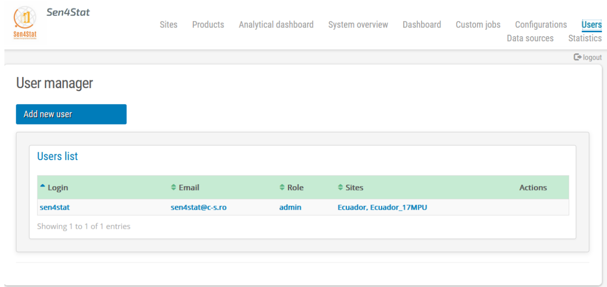
Figure 4-23. Users management
